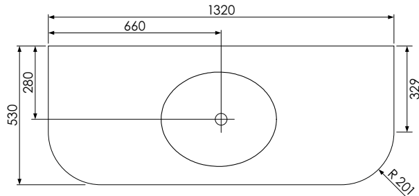
Worktop with single integral basin 650-XX-WT13253/25BCE
