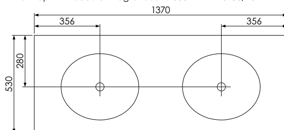
Worktop with double integral basins 650-XX-WT13753/25B2
