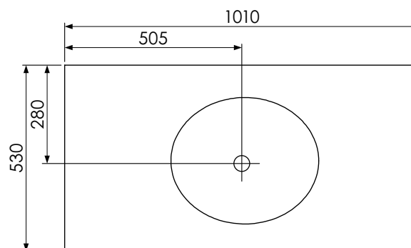
Worktop with single integral basin 650-XX-WT10153/25BM
