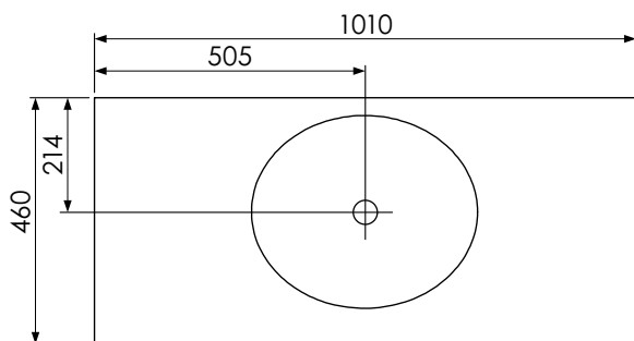
Worktop with single integral basin 650-XX-WT10146/25BM
