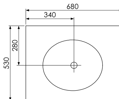
Worktop with single integral basin 650-XX-WT6853/25B
