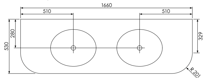
Worktop with double integral basins 650-XX-WT16653/V2C
