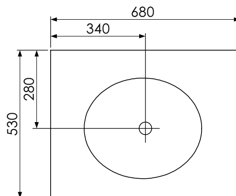
Worktop with single integral basin 650-XX-WT6853/25B
