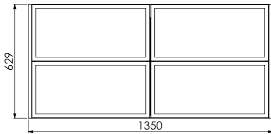
Worktop with double integral basins 650-XX-WT13746/25B2
