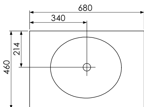
Worktop with single integral basin 650-XX-WT6846/25B
