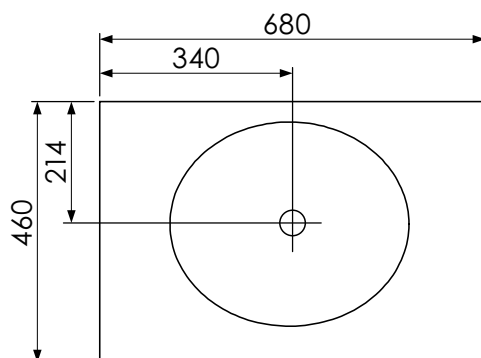
Worktop with single integral basin 650-XX-WT6846/25B
