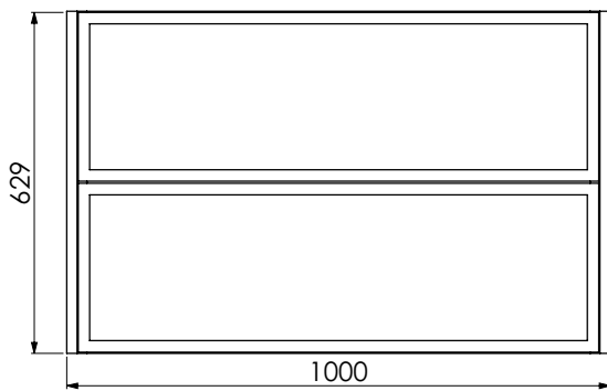
Worktop with single integral basin 650-XX-WT10146/25BM
